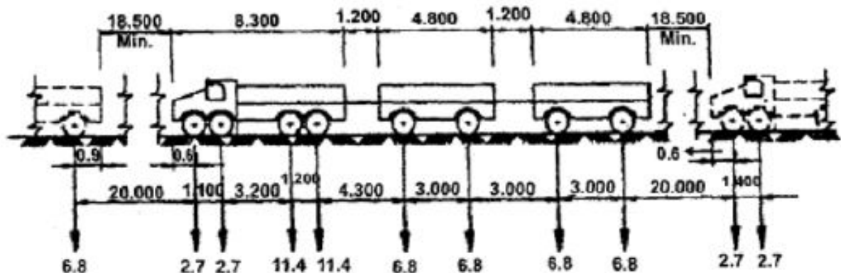
Fig. 2 IRC-Class A Train of vehicle
